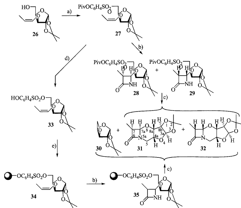
Scheme 3. a) \text{PivOC}_6\text{H}_4\text{SO}_2\text{Cl} ( 2 ), Py, DMAP; b) i. CSI, \text{Na}_2\text{CO}_3 , \text{CH}_2\text{Cl}_2 /toluene, -78 to -30 °C, 2–10 h, ii. Red-Al; c) BEMP or DBU, \Delta T , \text{CH}_3\text{CN} ; d) Na/MeOH; e) Wang resin ( 11 ), DEAD, TPP, \text{CH}_2\text{Cl}_2 , 48 h
