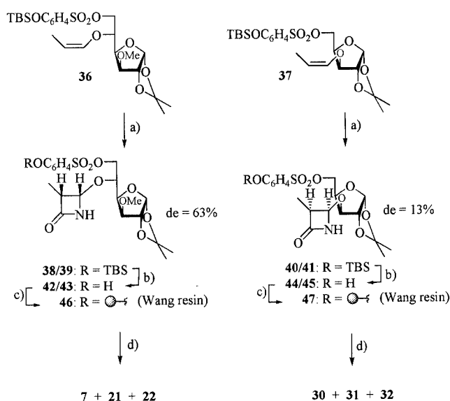
Scheme 4. a) \text{PivOC}_6\text{H}_4\text{SO}_2\text{Cl} ( 2 ), Py, DMAP; b) TBAB, THF, room temp., 15 min; c) Wang resin ( 11 ), DEAD, TPP, \text{CH}_2\text{Cl}_2 , 48 h; d) BEMP or DBU, \text{CH}_3\text{CN} , \Delta T , 1.5 h
